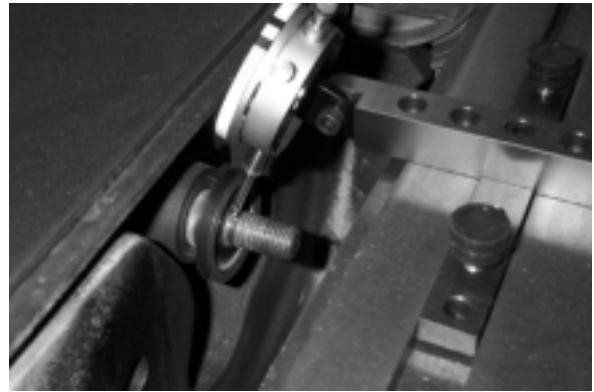
Check Arbor Runout and Bearing Play
