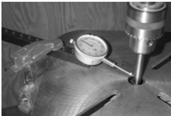
Check Drill Chuck Runout
