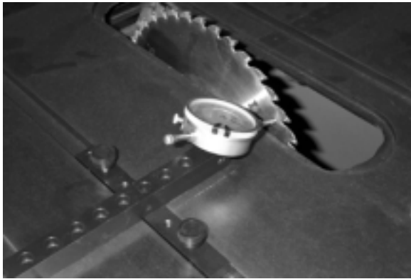
Check Table Saw Alignment
